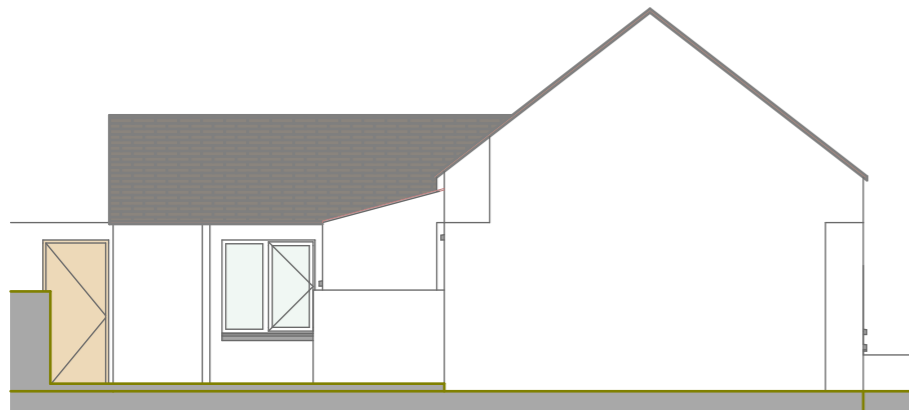
3 Side Elevation Existing 1:100
