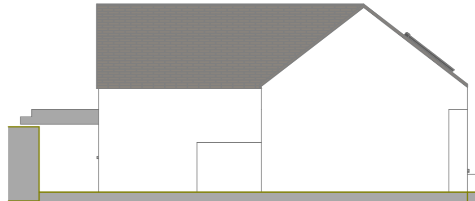
6 Side Elevation Proposed 1:100
