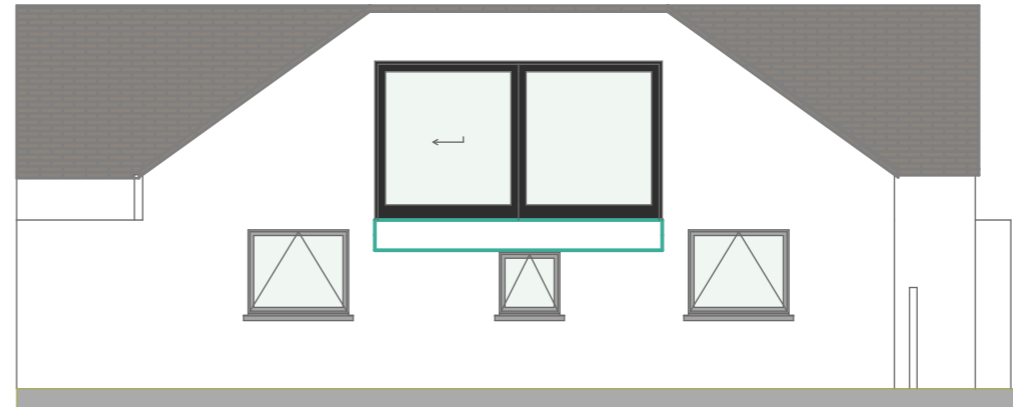
5 Rear Elevation Proposed 1:100
